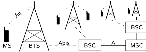
Fig. 1: The architecture of a GSM network.
