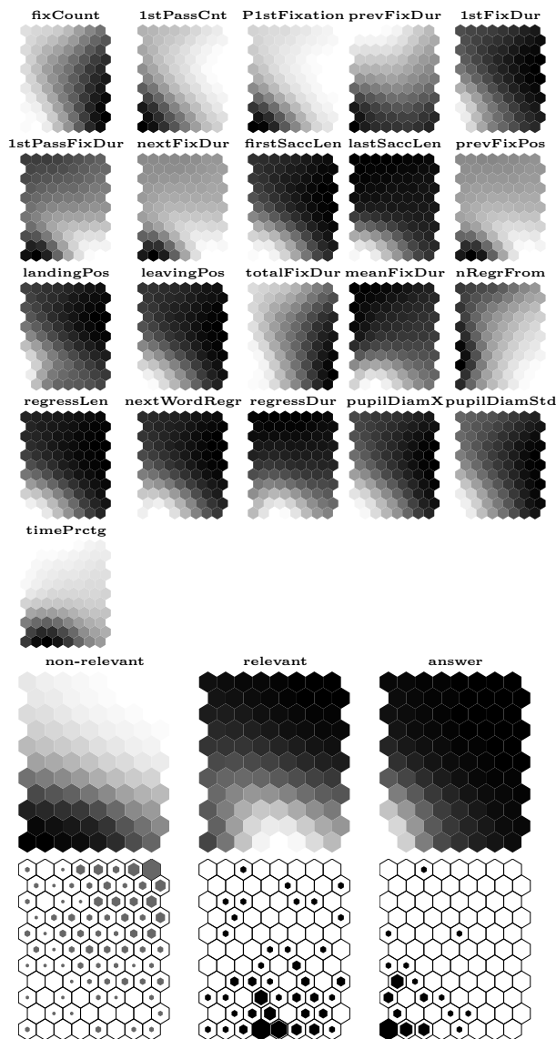
Figure 4: Above: Visualization of the relative contribution of each feature to the approximative Fisher metric at each SOM unit. Center: A plot of conditional probability densities in each node for non-relevant and relevant titles, and titles containing the answer. Below: Number of data points in each SOM unit.
