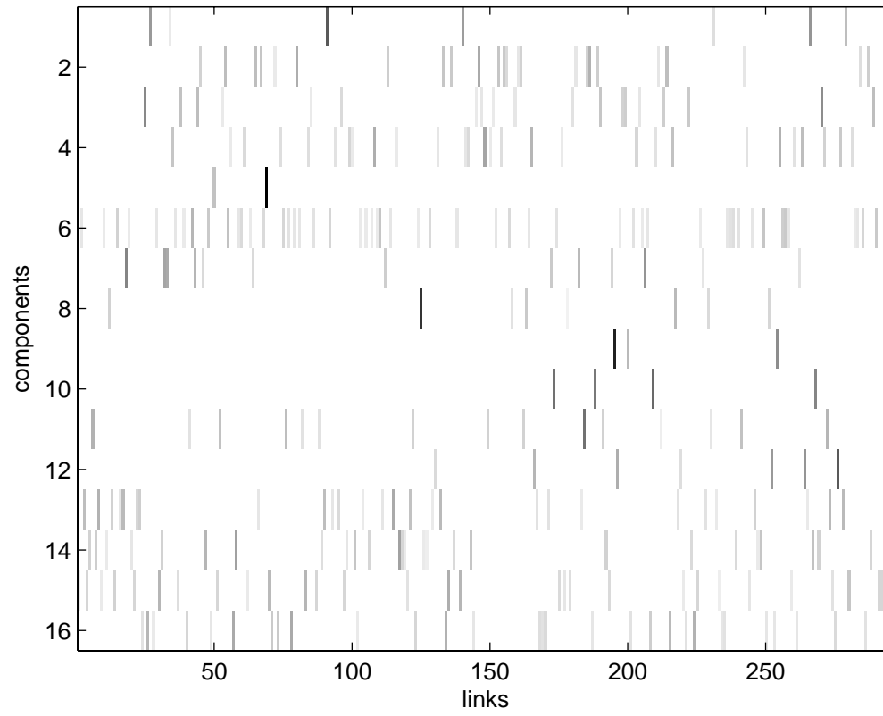
P-NMF projection matrix visualization
