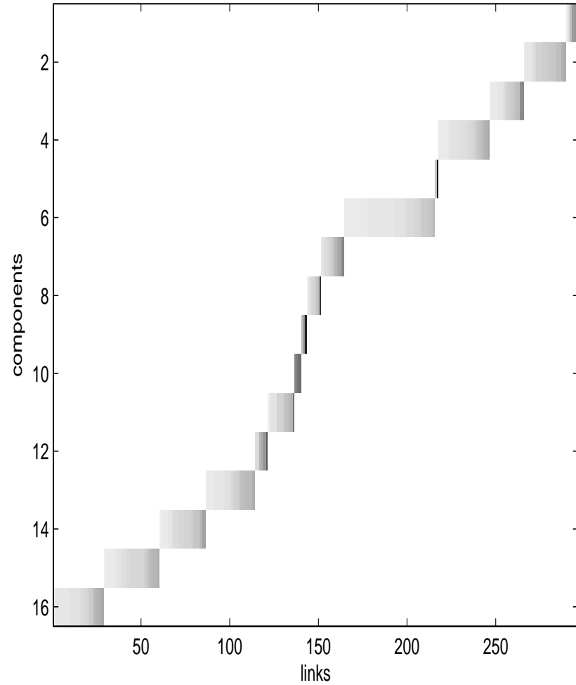
sorted P-NMF projection matrix
